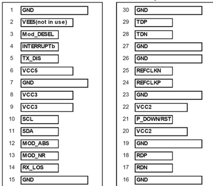
XFP Transceiver Electrical Pad Layout
